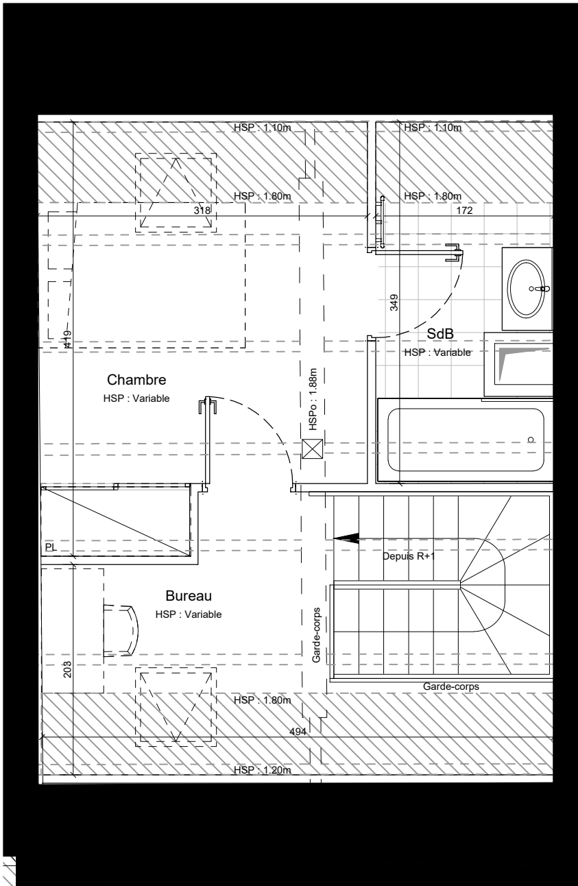
Plan combles
