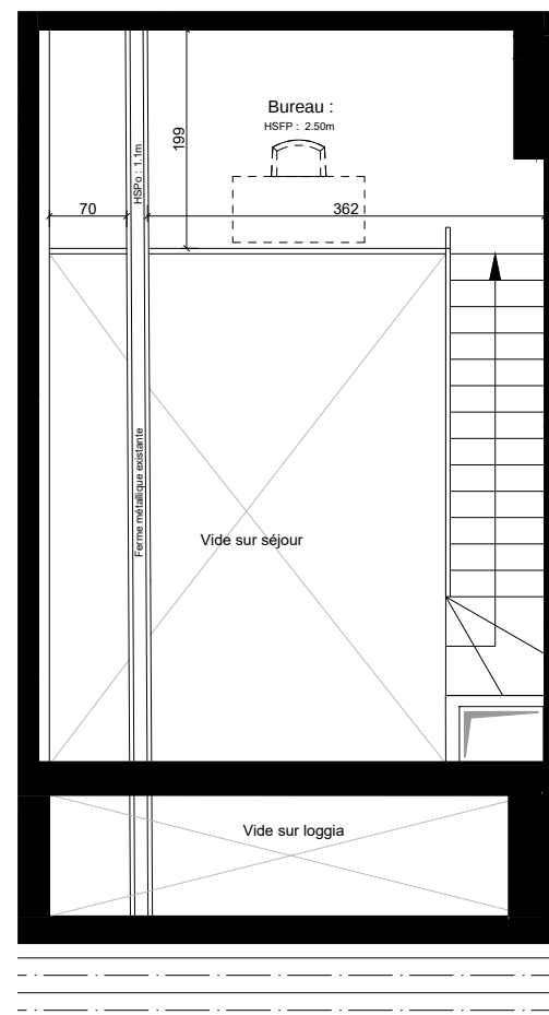
Plan Mezzanine
